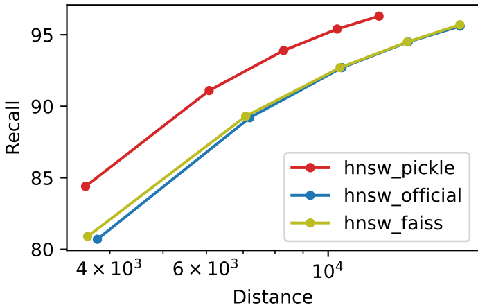
Recall vs Distance text2image_10M_M32_ef300_k100
