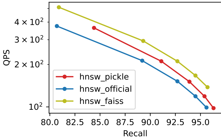
Recall vs QPS text2image_10M_M32_ef300_k100
