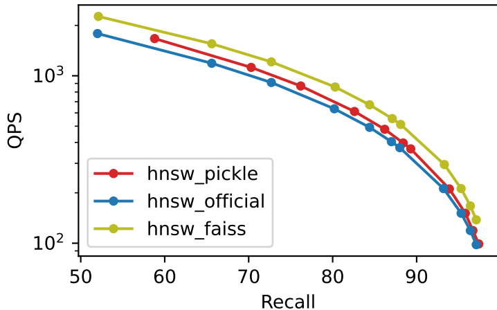
Recall vs QPS text2image_10M_M32_ef300_k10
