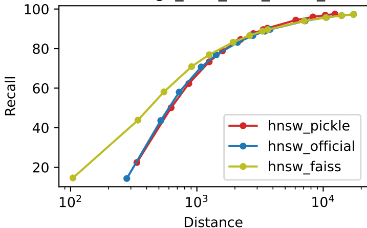
Recall vs Distance text2image_10M_M32_ef300_k1
