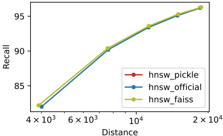
Recall vs Distance text2image_10M_M32_ef500_k100
