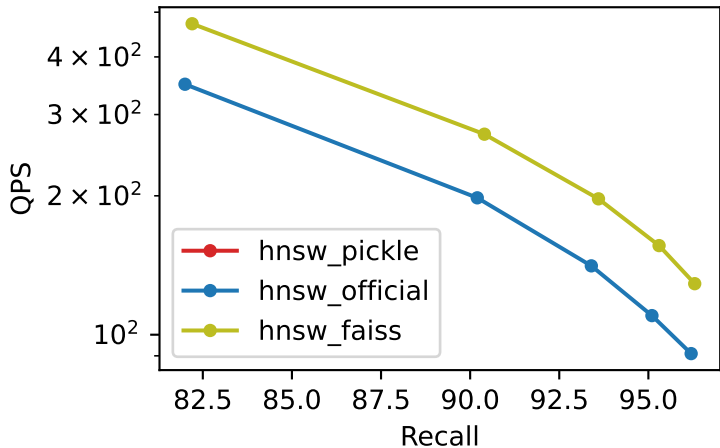
Recall vs QPS text2image_10M_M32_ef500_k100
