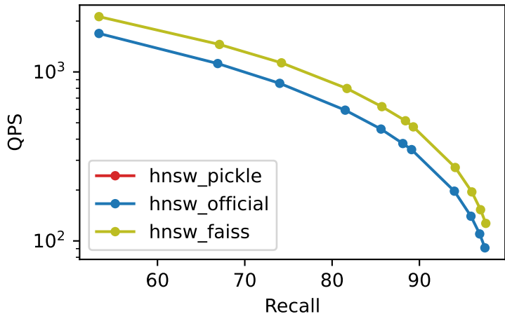
Recall vs QPS text2image_10M_M32_ef500_k10
