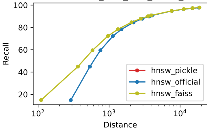
Recall vs Distance text2image_10M_M32_ef500_k1
