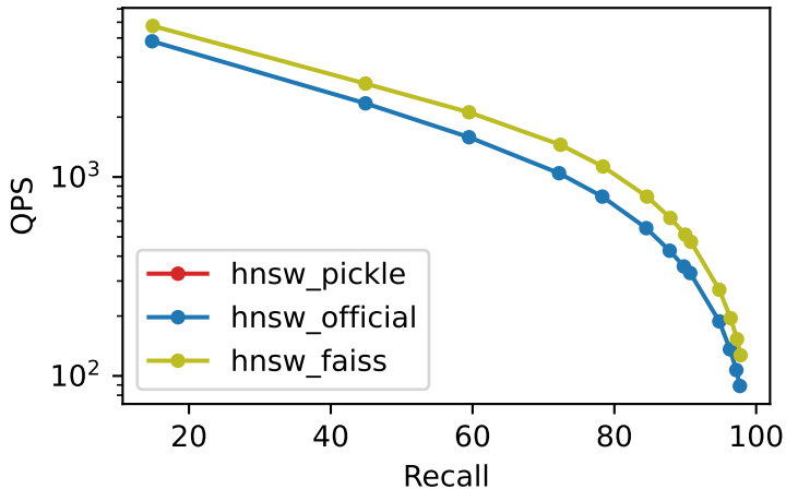
Recall vs QPS text2image_10M_M32_ef500_k1
