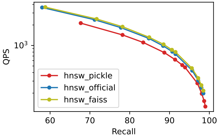
Recall vs QPS text2image_1M_M32_ef100_k10
