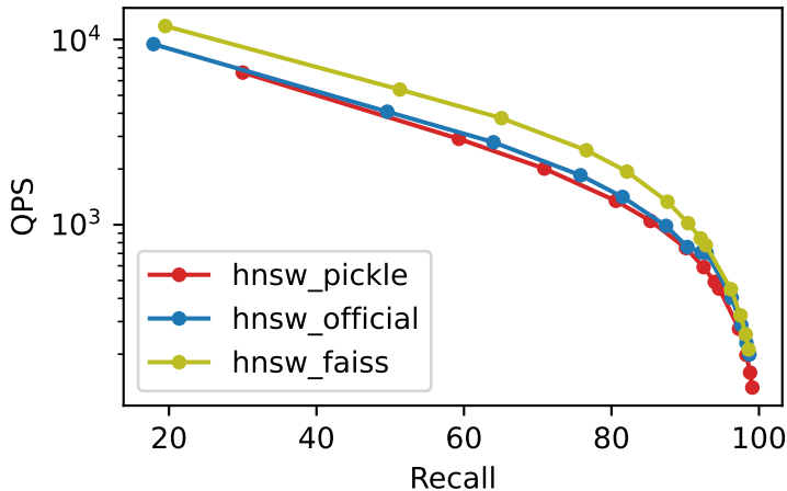
Recall vs QPS text2image_1M_M32_ef100_k1
