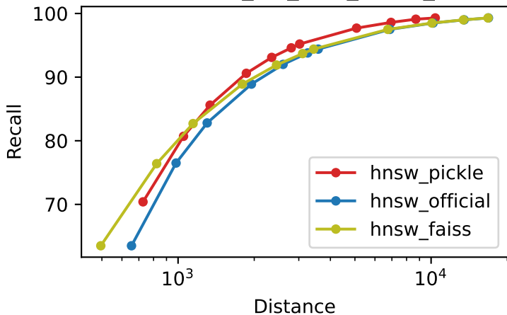
Recall vs Distance text2image_1M_M32_ef300_k10
