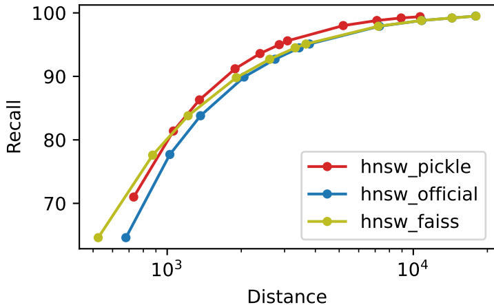
Recall vs Distance text2image_1M_M32_ef500_k10
