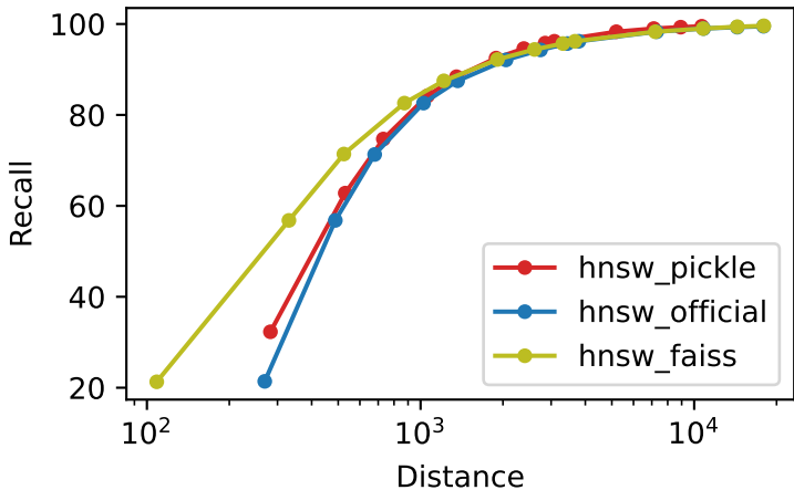
Recall vs Distance text2image_1M_M32_ef500_k1
