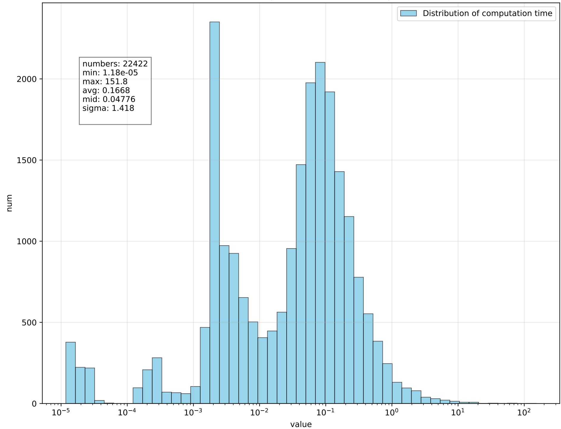
Distribution of Computation Time (X-axis Log Scale)
