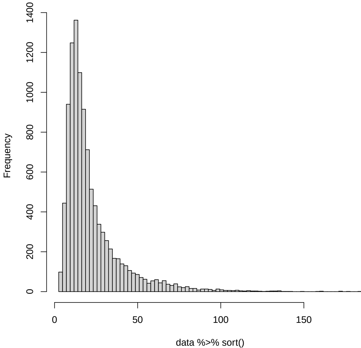
hist BUN
