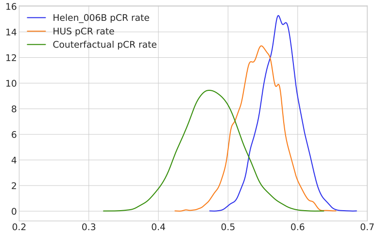
Figure 5: Estimated pCR rates for HELEN-006 B arm, HUS and HUS with baseline adjustment.
