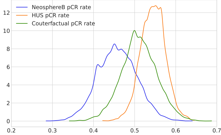
Figure 1: Estimated pCR rates for NeoSphere B arm, HUS and HUS with baseline adjustment.
