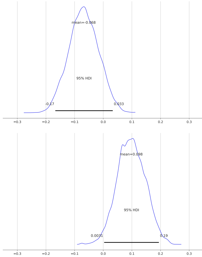
Figure 12: Top: Adjustment difference \Delta\hat{\theta}_{\text{adj}} and Bottom: residual difference \Delta\hat{\theta}_{\text{res}} for HELEN-006.
