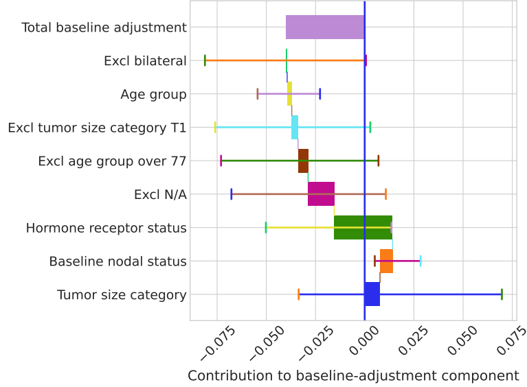
Figure 2: Shapley decomposition of the adjustment difference for the NeoSphere comparison. Bars represent mean Shapley contributions and error bars show 95% HDIs. Mean contributions sum to the total adjustment effect.
