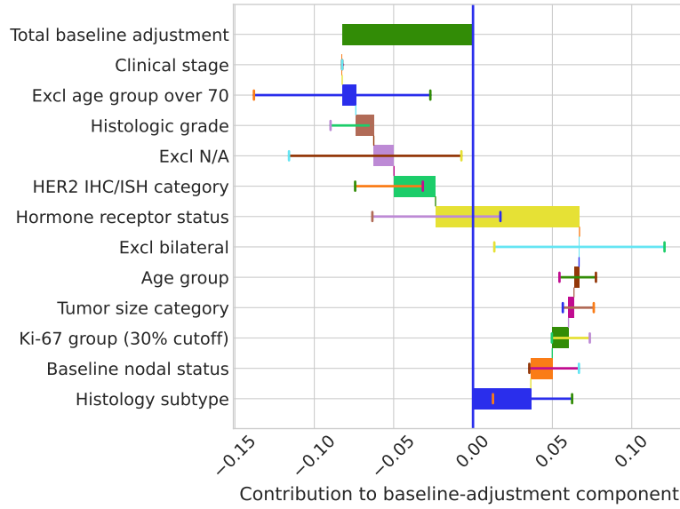
Figure 6: Shapley decomposition of the adjustment difference for the HELEN-006 comparison. Bars represent mean Shapley contributions and error bars show 95% HDIs. Mean contributions sum to the total adjustment effect.
