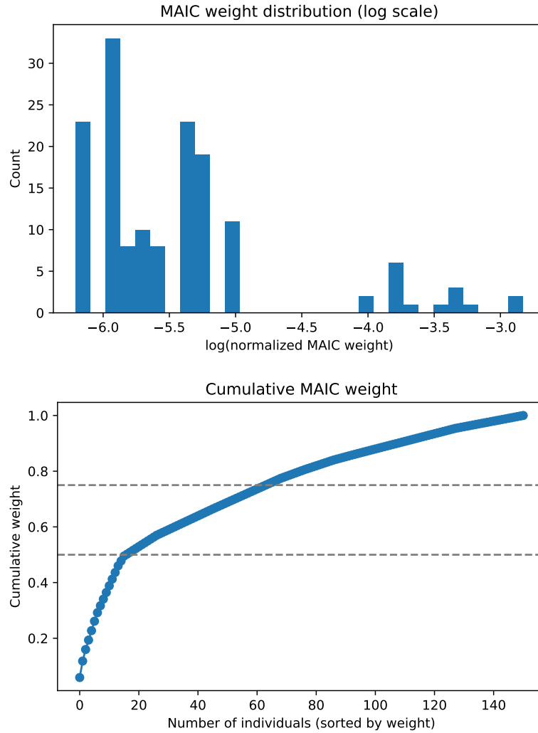
Figure 7: MAIC weight diagnostics for the NeoSphere comparison. Top panel: Histogram of individual log-weights from the MAIC model, illustrating a multimodal distribution with a small number of observations receiving relatively large weights. Bottom panel: Cumulative weight proportion as a function of the number of individuals, showing that the 20 highest-weighted individuals account for approximately 50% of the total weight.
