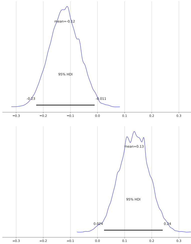
Figure 11: Top: Adjustment difference \Delta\hat{\theta}_{\text{adj}} and Bottom: residual difference \Delta\hat{\theta}_{\text{res}} for KRISTINE.
