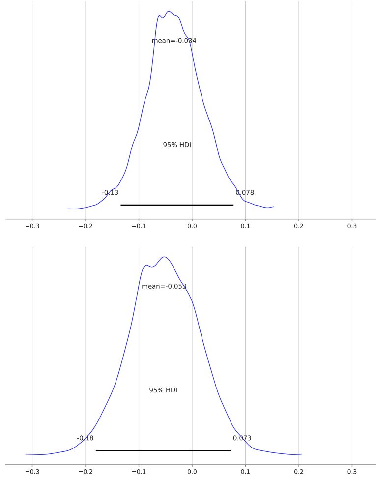
Figure 10: Posterior distributions of the adjustment difference \Delta\hat{\theta}_{\text{adj}} (top) and residual difference \Delta\hat{\theta}_{\text{res}} (bottom) for the NeoSphere comparison.
