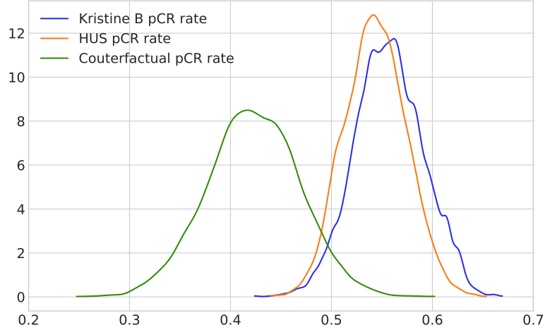
Figure 3: Estimated pCR rates for KRISTINE B arm, HUS and HUS with baseline adjustment.
