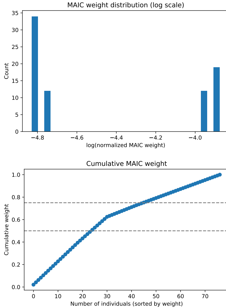
Figure 8: MAIC weight diagnostics for the KRISTINE comparison. Top panel: Distribution of individual log-weights from the MAIC model. Bottom panel: Cumulative weight proportion as a function of the number of individuals.
