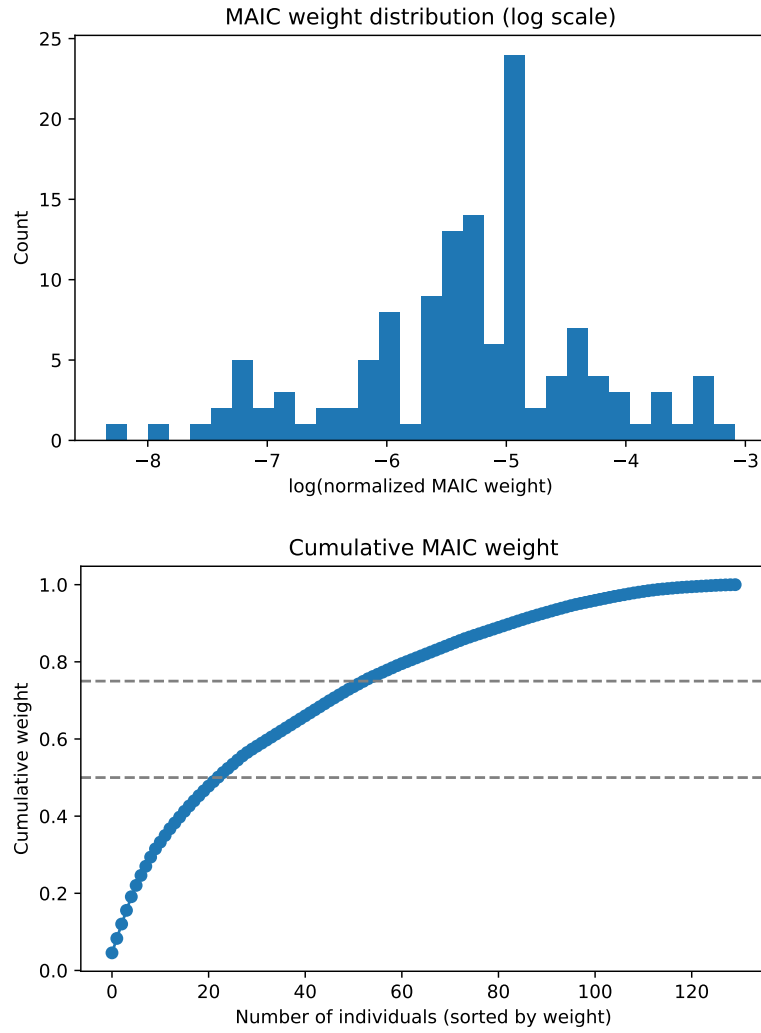
Figure 9: MAIC weight diagnostics for the HELEN-006 comparison. Top panel: Distribution of individual log-weights from the MAIC model. Bottom panel: Cumulative weight proportion as a function of the number of individuals.
