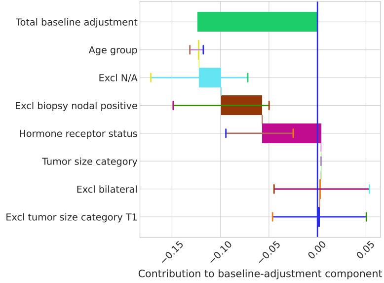
Figure 4: Shapley decomposition of the adjustment difference for the KRISTINE comparison. Bars represent mean Shapley contributions and error bars show 95% HDIs. Mean contributions sum to the total adjustment effect.
