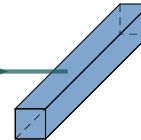
Embedding 2
