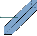
Embedding 3
