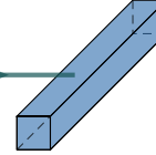
Embedding 1
