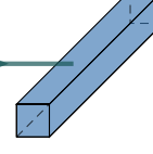
Embedding 5
