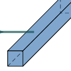
Embedding 4
