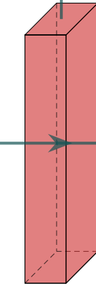
Feature Map 3
