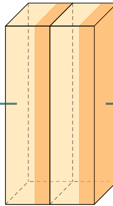
FPN + Conv
