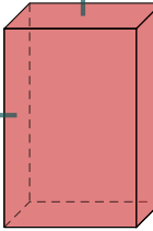
Feature Map 4
