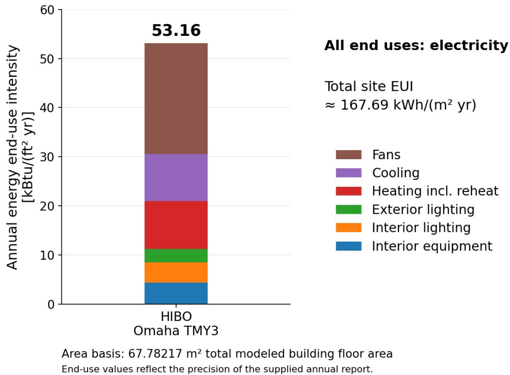
Figure 7-1. Annual site-energy end-use intensity for HIBO, Omaha TMY3. [5]
