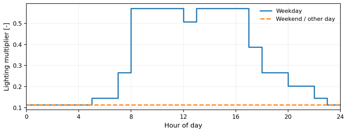
Figure 5-2. Interior lighting schedule. The entered weekday maximum is about 0.571 of design power, not 1.0. [1]
