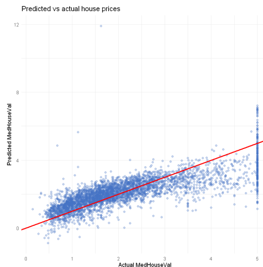
Predicted versus actual house prices on the test set.
