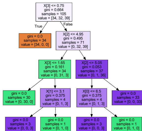
A trained decision tree, showing the splits learned for classification.
