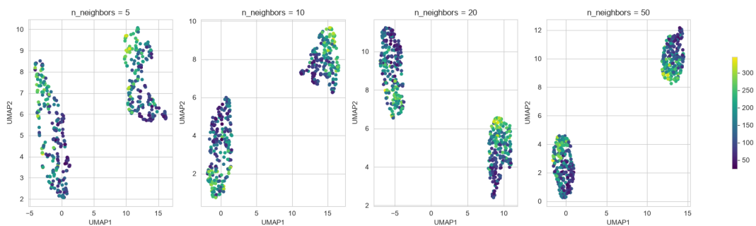
Low-dimensional embeddings of the diabetes data.
