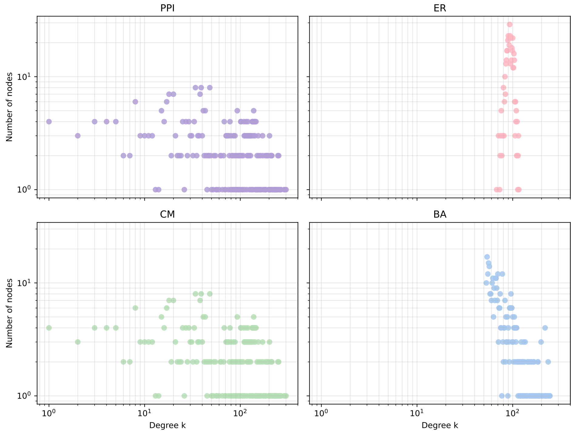
Figure 1: Degree distribution (log-log)
