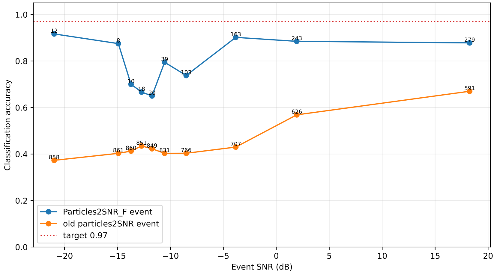
Available event accuracy by SNR
