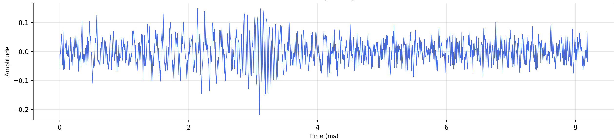
Panel 1: Original Signal
