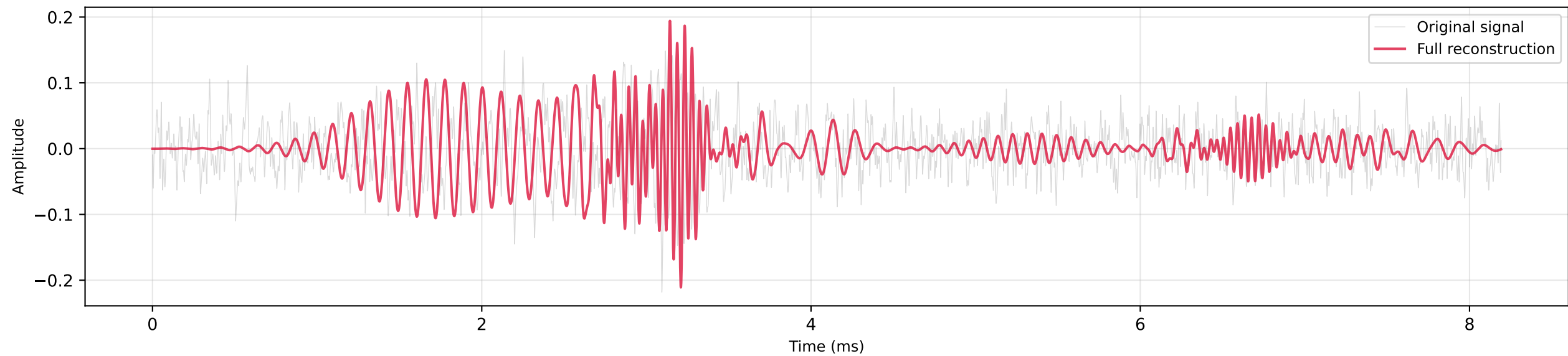
Panel 3: Full Reconstruction
