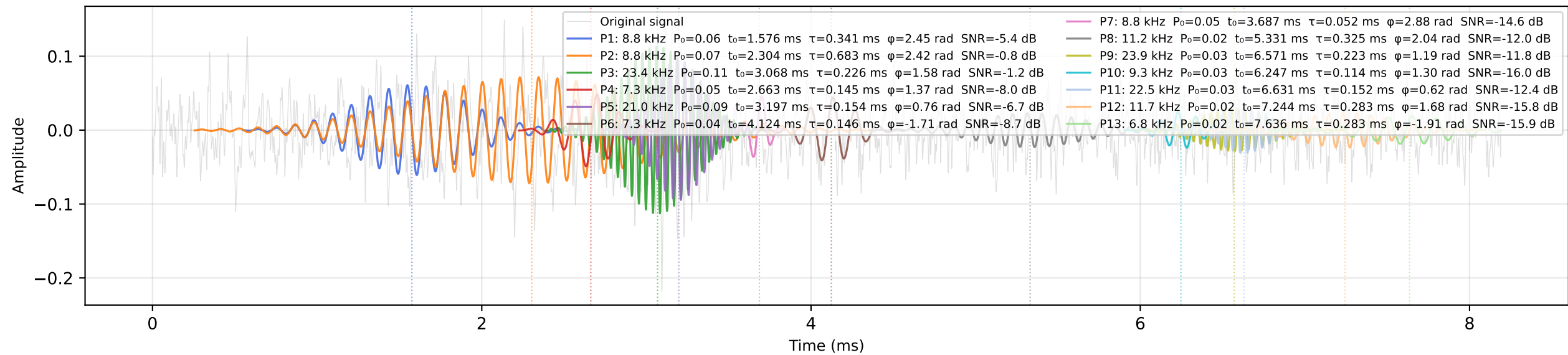
Panel 2: All Particles Overlay ( \pm 3\sigma , 99.7%)
