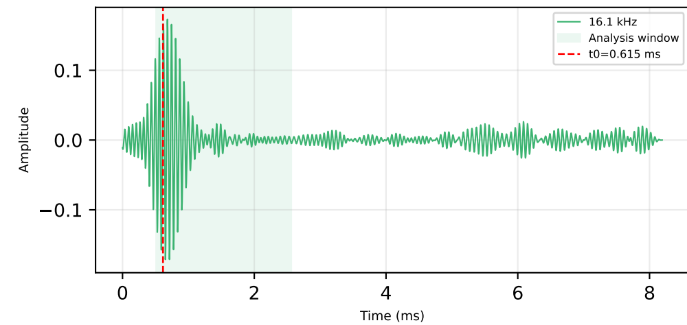
Narrow bandpass - particle 1
