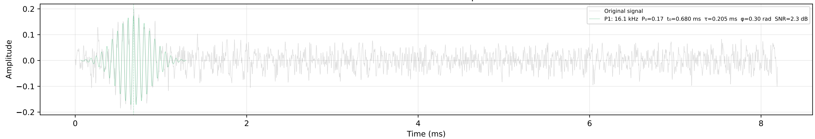
Cosine-Gaussian estimated particles
