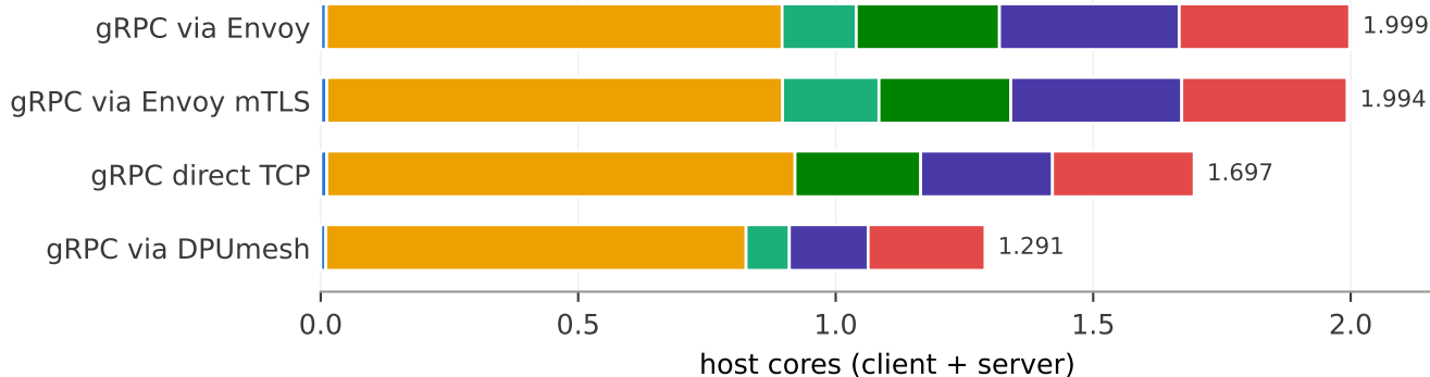
(b) L7 unary gRPC, 64 B at 24 k/s
