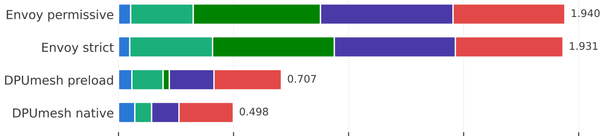
(b) L7 unary gRPC, 64 B at 24 k/s
