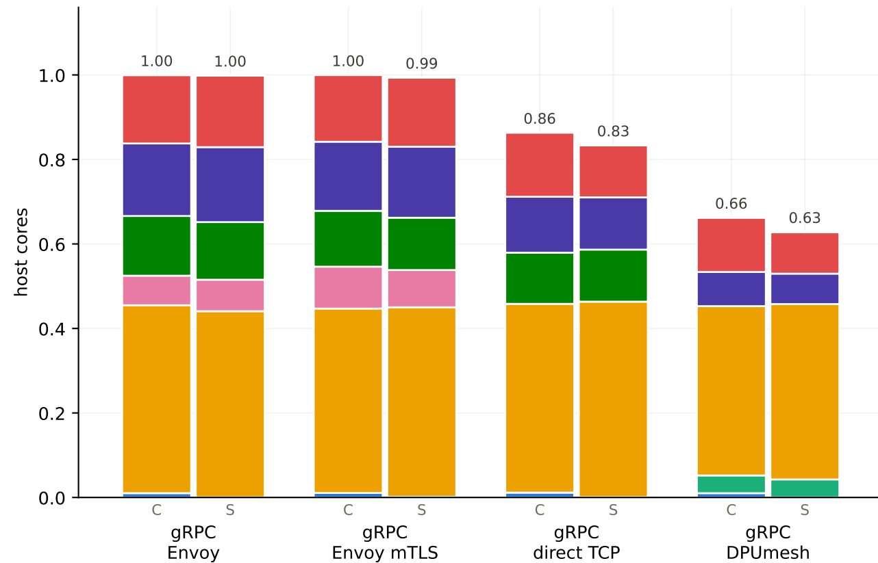
64 B frame, 24k/s offered
