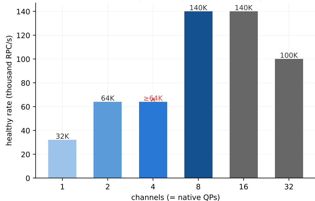
Capacity served with the median bounded (arrow: still rising at the top of the measured grid)
