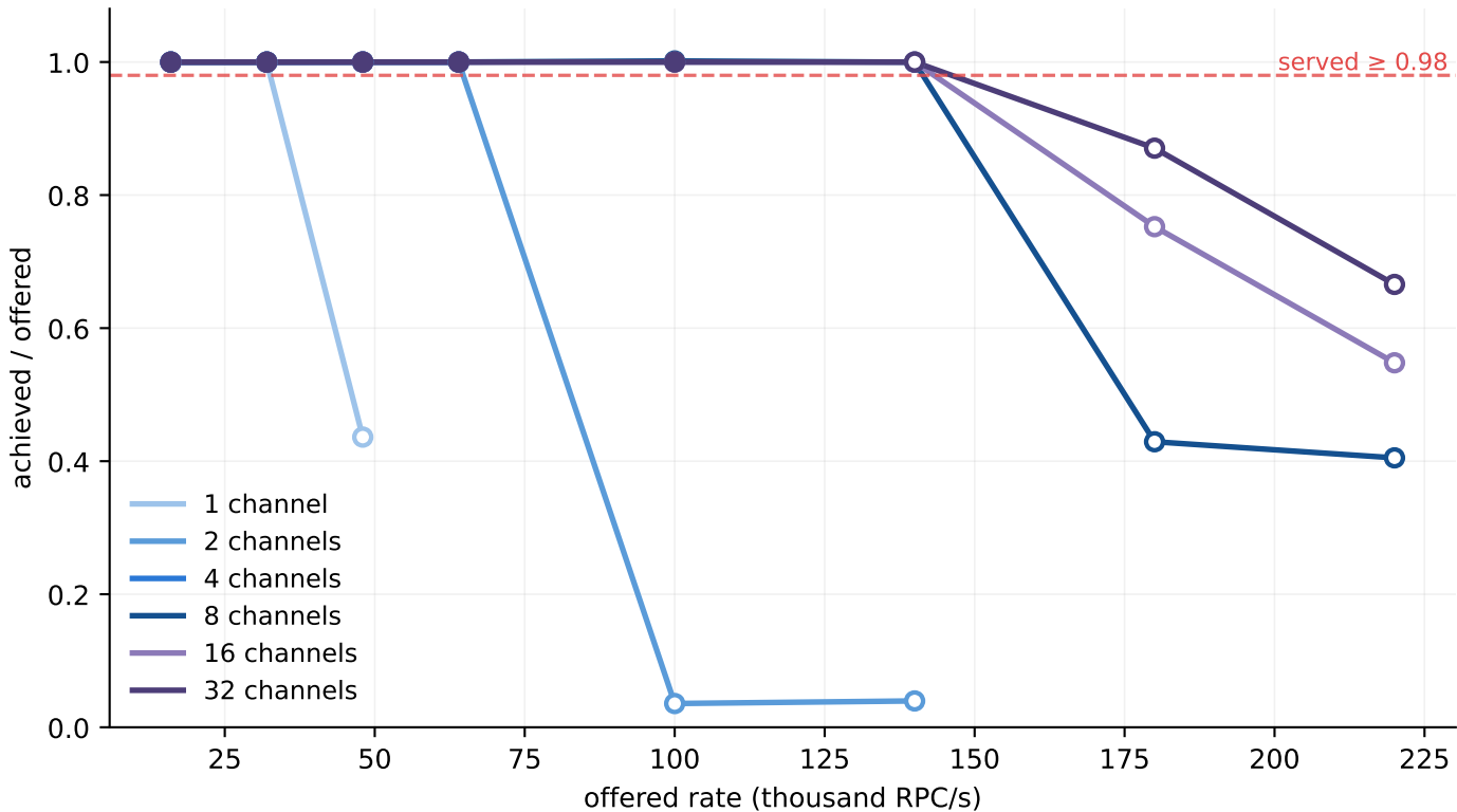
What each channel count delivers (hollow marker: median above 1000 \mu s)
