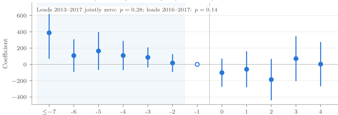
c Green patent stock (firm level)
