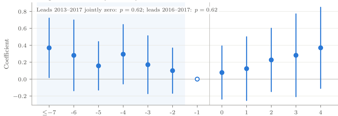
b Emission intensity, tCO 2 e per $M output (sector level)
