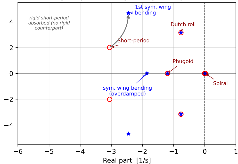
(b) Flight-dynamics region (rigid-body modes)
