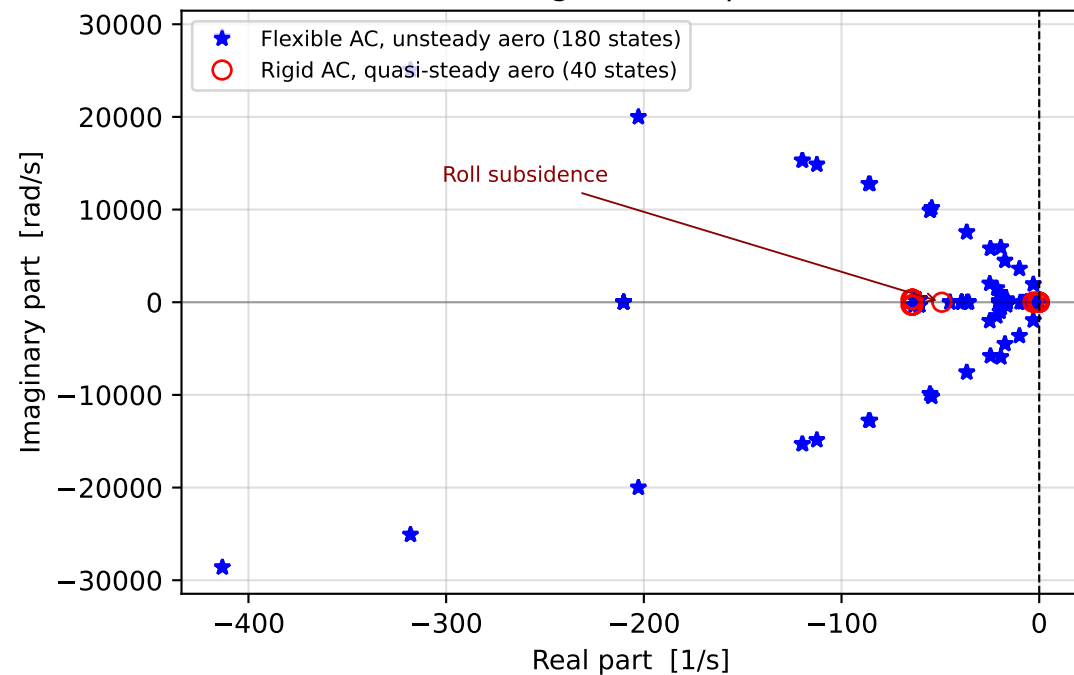
(a) Full eigenvalue spectrum
