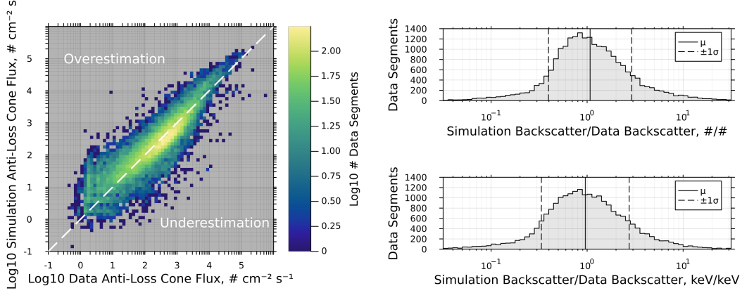
Figure 9. Left: Anti-loss cone electron flux predicted by lookup tables derived from our Monte Carlo simulation vs. ELFIN-measured anti-loss cone electron flux for all ELFIN data segments that were simulated in Section 4. The dashed white line indicates where predicted backscatter was equal to ELFIN-measured backscatter. Energy backscatter follows the same pattern and is not included for brevity (see Supporting Information). Right, top: 1-dimensional histogram plotting total number of electrons in the anti-loss cone predicted by the simulation divided by the same quantity measured by ELFIN. One standard deviation is a factor of 2.714. Right, bottom: 1-dimensional histogram plotting total energy in the anti-loss cone predicted by the simulation divided by the same quantity measured by ELFIN. One standard deviation is a factor of 2.868. This is based on 63 hours (69,510 spacecraft spins) of data.
