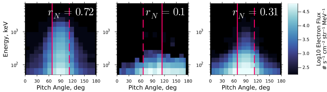
Figure 6. ELFIN-measured fluxes for data segments at three different levels of backscatter. Left: A data segment with little filling of the loss cone and high backscatter ratio. Center: A data segment with strong loss cone filling and low backscatter ratio. Right: A data segment with partial loss cone filling and an intermediate backscatter ratio. Solid lines indicate the pitch angle of the 100 km loss cone, and dashed lines indicate the conjugate anti-loss cone pitch angle. The center panel was recorded in the Southern hemisphere, thus \alpha_{LC} > \alpha_{ALC} .
