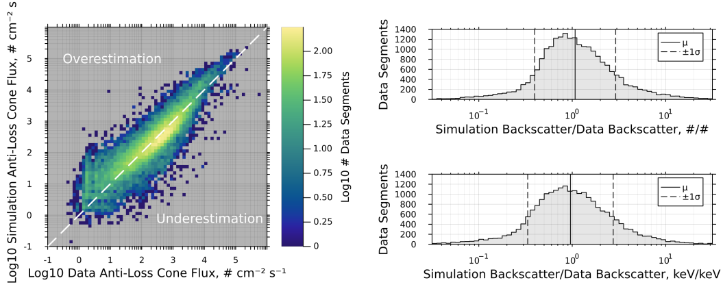
Figure 9. Left: Anti-loss cone electron flux predicted by lookup tables derived from our Monte Carlo simulation vs. ELFIN-measured anti-loss cone electron flux for all ELFIN data segments that were simulated in Section 4. The dashed white line indicates where predicted backscatter was equal to ELFIN-measured backscatter. Energy backscatter follows the same pattern and is not included for brevity (see Supporting Information). Right, top: 1-dimensional histogram plotting total number of electrons in the anti-loss cone predicted by the simulation divided by the same quantity measured by ELFIN. One standard deviation is a factor of 2.714. Right, bottom: 1-dimensional histogram plotting total energy in the anti-loss cone predicted by the simulation divided by the same quantity measured by ELFIN. One standard deviation is a factor of 2.868. This is based on 63 hours (69,510 spacecraft spins) of data.
