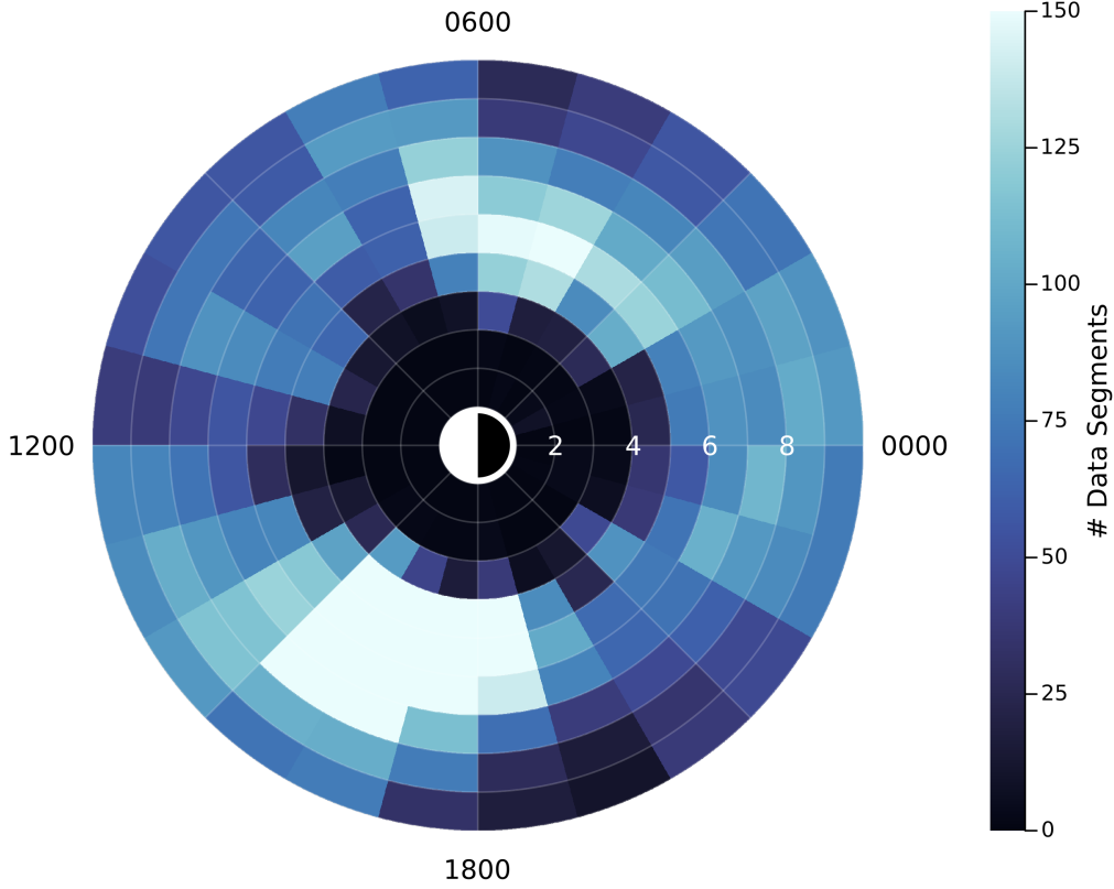
Figure 3. L-MLT coverage of the ELFIN dataset from which we will calculate backscatter ratios. This dataset encompasses [TODO: ] hours ([TODO: ] spacecraft spins) of ELFIN data collected over 2 years. L and MLT are calculated using the T87 magnetic field model.
