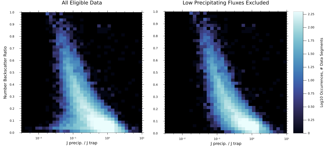
Figure 5. Number backscatter ratio vs. loss cone filling strength derived from [TODO: ] hours ([TODO: ] spacecraft spins) of ELFIN data. Any measurement of backscatter ratio with absolute uncertainty greater than \sigma \approx 0.025 was discarded. Left: Results using data as previously described. Right: Measurements with precipitating flux less than 10^{3.5} electrons- \text{cm}^{-2}\text{-s}^{-1} removed to avoid artificially lowered backscatter ratios due to backscattered fluxes falling below the instrument noise floor. Energy backscatter ratio has a similar pattern to number backscatter ratio and is not shown for brevity.
