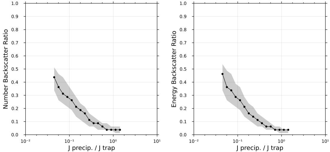
Figure 2: Median backscatter (black line) as well as the 25th and 75th percentile (grey ribbon below and above, respectively) as a function of precipitation strength. Left panel shows the number backscatter ratio r_N , right panel shows the energy backscatter r_E .
