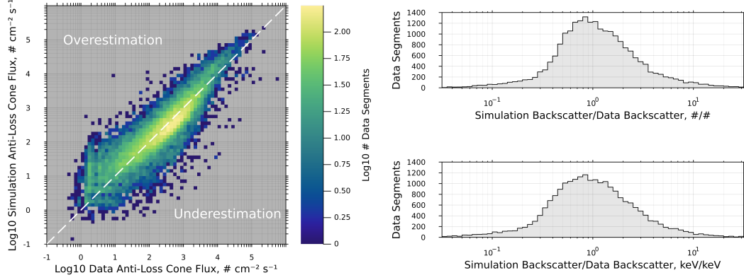
Figure 9. Left: Anti-loss cone electron flux predicted by lookup tables derived from our Monte Carlo simulation vs. ELFİN-measured anti-loss cone electron counts for all ELFİN data segments that were simulated in Section 4. The dashed white line indicates where predicted backscatter was equal to ELFİN-measured backscatter. Energy backscatter follows the same pattern and is not included for brevity. Right, top: 1-dimensional histogram plotting total number of electrons in the anti-loss cone predicted by the simulation divided by the same quantity measured by ELFİN. Right, bottom: 1-dimensional histogram plotting total energy in the anti-loss cone predicted by the simulation divided by the same quantity measured by ELFİN. This is based on 63 hours (69,510 spacecraft spins) of data.
