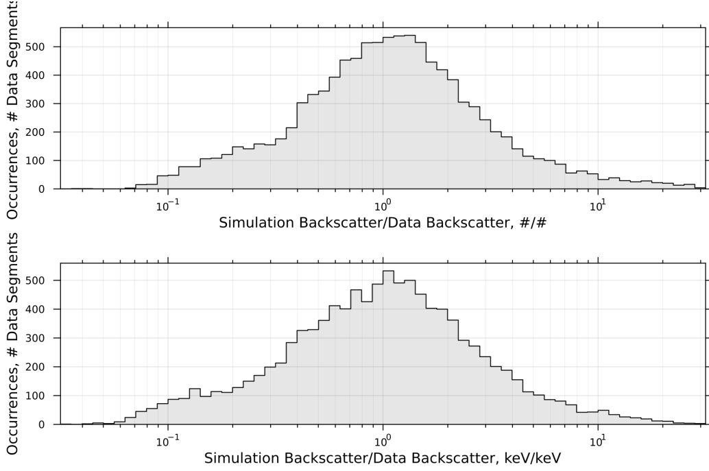
Figure 9. Anti-loss cone electron count predicted by lookup tables derived from our Monte Carlo simulation divided by ELFIN-measured anti-loss cone electron counts for all ELFIN data segments that were analyzed in Section 4. This is based on 26 hours (33,366 spacecraft spins) of data.
