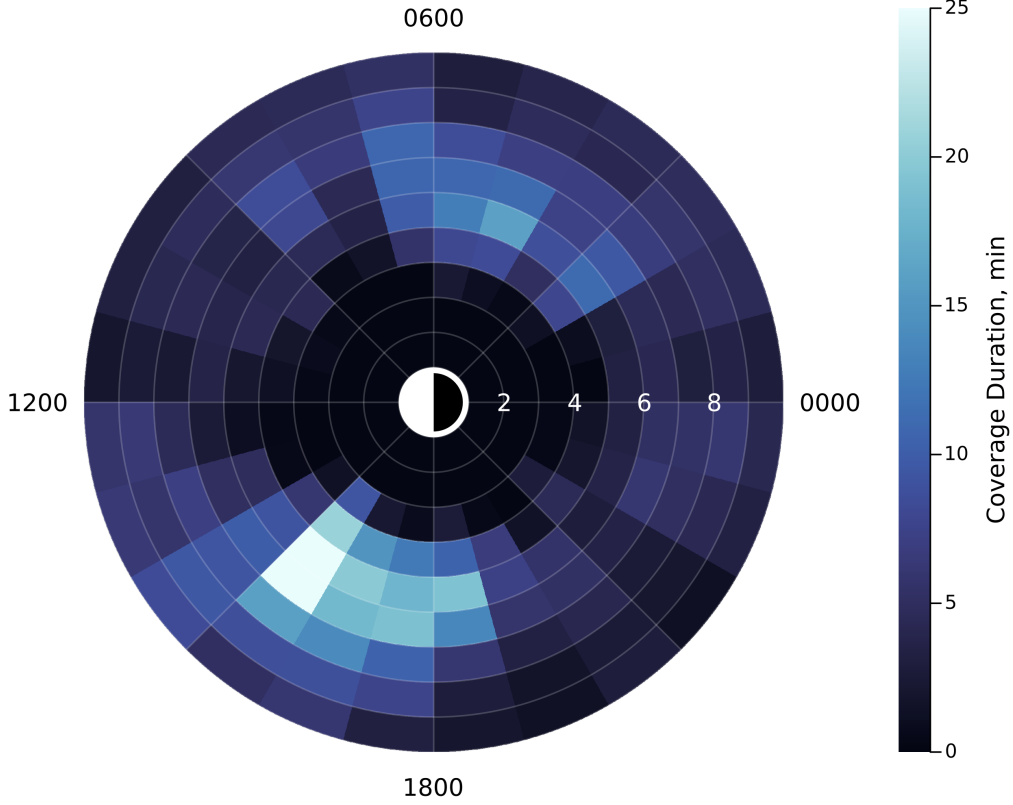
Figure 3. L-MLT coverage of the ELFIN dataset from which we will calculate backscatter ratios. This dataset encompasses 26 hours (33,366 spacecraft spins) of ELFIN data collected over 2 years. L and MLT are calculated using the T87 magnetic field model.
