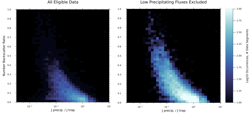
Figure 5. Number backscatter ratio vs. loss cone filling strength derived from 26 hours (33,366 spacecraft spins) of ELFIN data. Any measurement of backscatter ratio with absolute uncertainty greater than \sigma \approx 0.025 was discarded. Left: Results using data as previously described. Right: Measurements with precipitating flux less than 10^{3.5} electrons-cm ^{-2} -s ^{-1} removed to avoid artificially lowered backscatter ratios due to backscattered fluxes falling below the instrument noise floor. Energy backscatter ratio has a similar pattern to number backscatter ratio and is not shown for brevity.
