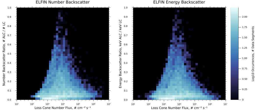
Figure 4. Backscatter ratios derived from 26 hours (33,366 spacecraft spins) of ELFIN data. Backscatter ratio is defined as the total electron number or energy measured in the anti-loss cone divided by the total number or energy measured in the loss cone. Any measurement of backscatter ratio with absolute uncertainty greater than \sigma \approx 0.025 was discarded.
