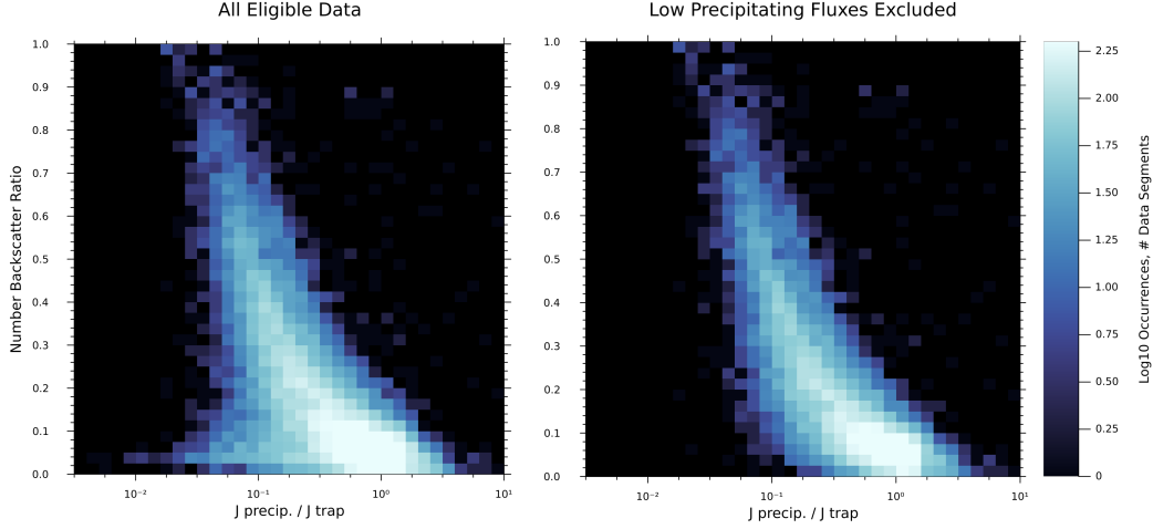
Figure 5. Number backscatter ratio vs. loss cone filling strength derived from [TODO: 63 hours (69,510 spacecraft spins)] of ELFIN data. Any measurement of backscatter ratio with absolute uncertainty greater than \sigma \approx 0.025 was discarded. Left: Results using data as previously described. Right: Measurements with precipitating flux less than 10^{2.75} electrons-cm -2 -s -1 removed to avoid artificially lowered backscatter ratios due to backscattered fluxes falling below the instrument noise floor. Energy backscatter ratio has a similar pattern to number backscatter ratio and is not shown for brevity.
