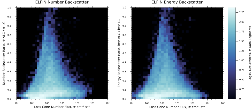
Figure 4. Backscatter ratios derived from [TODO: 63 hours (69,510 spacecraft spins)] of ELFIN data. Backscatter ratio is defined as the total electron number or energy measured in the anti-loss cone divided by the total number or energy measured in the loss cone. Any measurement of backscatter ratio with absolute uncertainty greater than \sigma \approx 0.025 was discarded.
