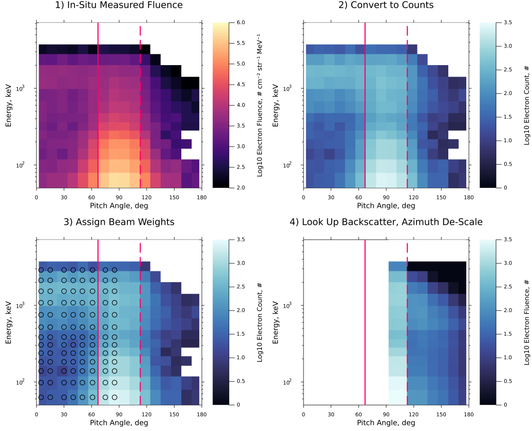
Figure 8. Illustration of the procedure used to fit Geant4 lookup tables to ELFIN data. Solid lines mark the loss cone pitch angle and dashed lines mark the anti-loss cone pitch angle. [TODO: 1) ELFIN-recorded fluxes are integrated over time for a given data segment to produce differential directional fluence. 2) Each recording bin is multiplied by its energy span and instrument geometric factor to produce measured electron counts. 3) Each data bin in the loss cone is scaled by azimuthal field of view (see text) and assigns its number of counts as a weight to the nearest energy and pitch angle for which a backscatter lookup table exists. Circular markers indicate the location of these lookup tables, and their color indicates their weight in electron counts. Lookup tables with zero weight are not shown for clarity. 4) Backscatter lookup tables are summed by their total weights, de-scaled in azimuthal field of view (see text), and returned.]
