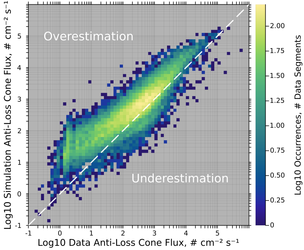
Figure 8. Anti-loss cone electron flux predicted by lookup tables derived from our Monte Carlo simulation vs. ELFIN-measured anti-loss cone electron counts for all ELFIN data segments that were simulated in Section 4. This is based on 63 hours (69,510 spacecraft spins) of data.
