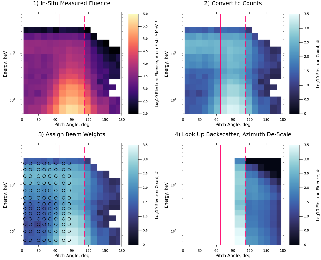
Figure 7. Illustration of the procedure used to fit Geant4 lookup tables to ELFIN data. Solid lines mark the loss cone pitch angle and dashed lines mark the anti-loss cone pitch angle. 1) ELFIN-recorded fluxes are integrated over time for a given data segment to produce differential directional fluence. 2) Each recording bin is multiplied by its energy span and instrument geometric factor to produce measured electron counts. 3) Each data bin in the loss cone is scaled by azimuthal field of view (see text) and assigns its number of counts as a weight to the nearest energy and pitch angle for which a backscatter lookup table exists. Circular markers indicate the location of these lookup tables, and their color indicates their weight in electron counts. Lookup tables with zero weight are not shown for clarity. 4) Backscatter lookup tables are summed by their total weights, de-scaled in azimuthal field of view (see text), and returned.
