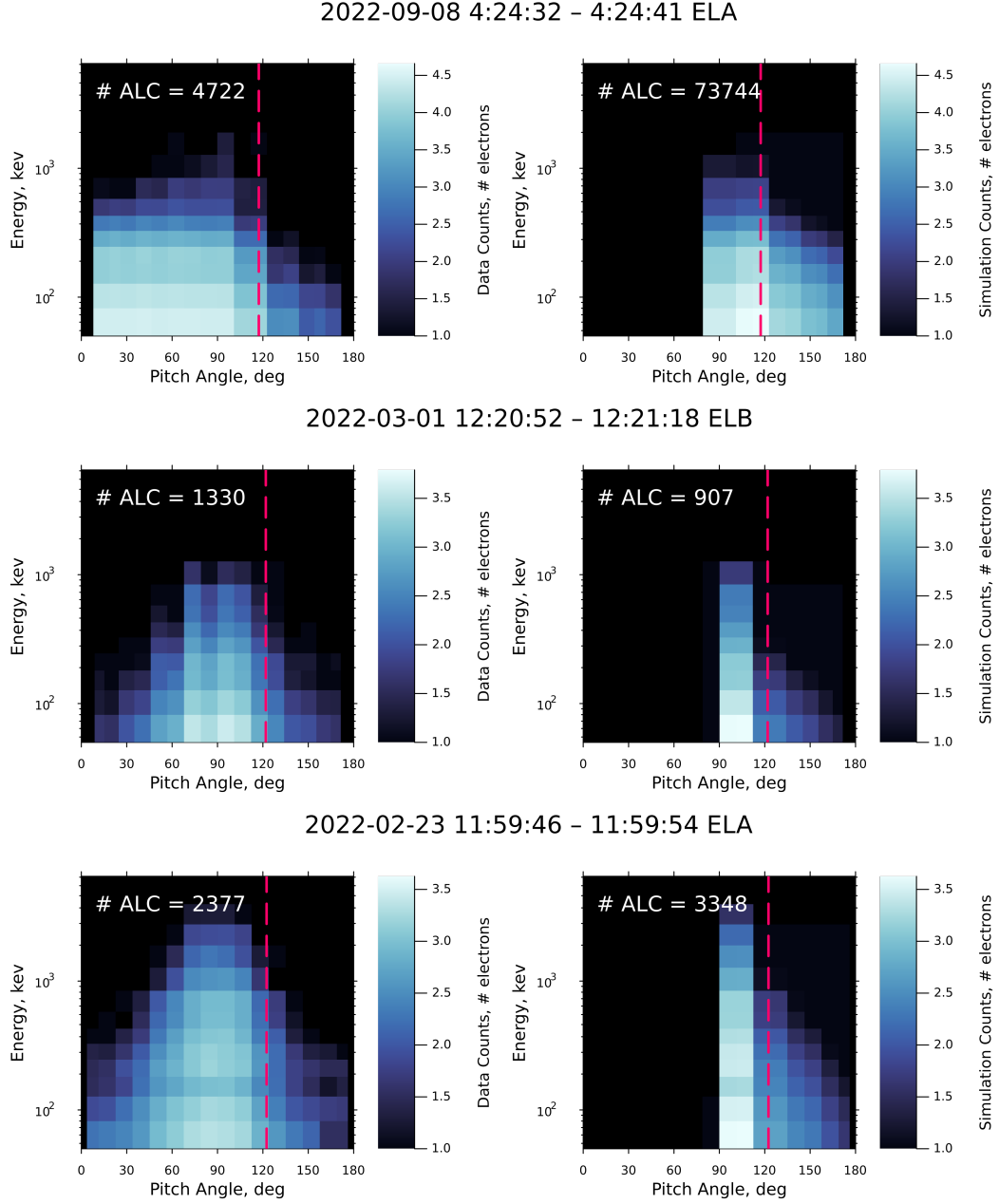
Figure 9. Examples of three data segments comparing ELFİN-recorded counts to model predictions. The dashed line is the pitch angle used to define the anti-loss cone, including the standoff angle of half of ELFİN’s FOV to ensure no contamination from the trapped region. The annotation “# ALC” shows the number of counts recorded in the anti-loss cone for each distribution. The top row shows a case where the model overestimates backscattered counts, the middle row shows slight underestimation, and the bottom row shows agreement.
