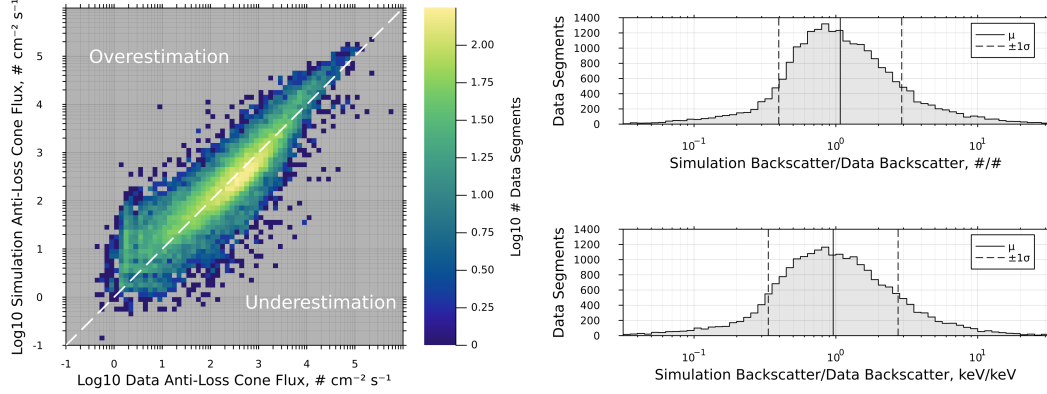
Figure 9. Left: Anti-loss cone electron flux predicted by lookup tables derived from our Monte Carlo simulation vs. ELFIN-measured anti-loss cone electron flux for all ELFIN data segments that were simulated in Section 4. The dashed white line indicates where predicted backscatter was equal to ELFIN-measured backscatter. Energy backscatter follows the same pattern and is not included for brevity (see Supporting Information for that figure). Right, top: 1-dimensional histogram plotting total number of electrons in the anti-loss cone predicted by the simulation divided by the same quantity measured by ELFIN. One standard deviation is a factor of 2.714. Right, bottom: 1-dimensional histogram plotting total energy in the anti-loss cone predicted by the simulation divided by the same quantity measured by ELFIN. One standard deviation is a factor of 2.868. This is based on 63 hours (69,510 spacecraft spins) of data.
