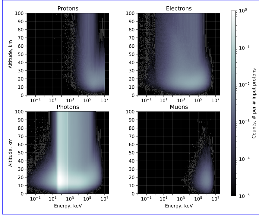
Figure 2. Example simulated energy spectra as a function of altitude for protons ( top left ), electrons ( center top right ), and photons ( bottom left ), and muons ( bottom right ). These spectra are the response to an input beam of 10^5 protons at 1.11 GeV injected with isotropic downgoing incidence into an MSIS atmosphere at 450 km.
