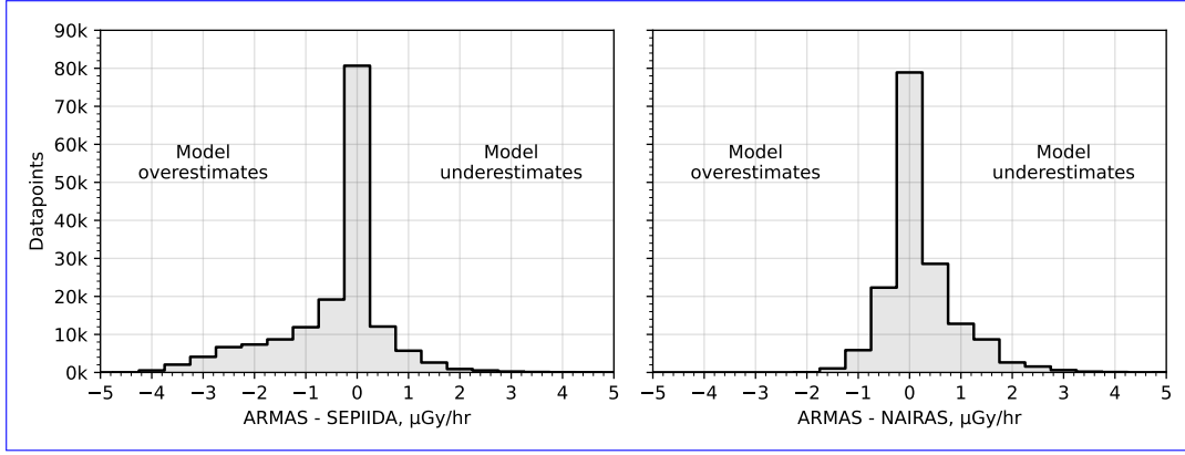
Figure 5. Left: Residuals between our GCR dose rate predictions and ARMAS data for all conjunction dates with AMS-02. Right: Residuals between NAIIRAS v1 predictions and ARMAS data for the same set of dates.
