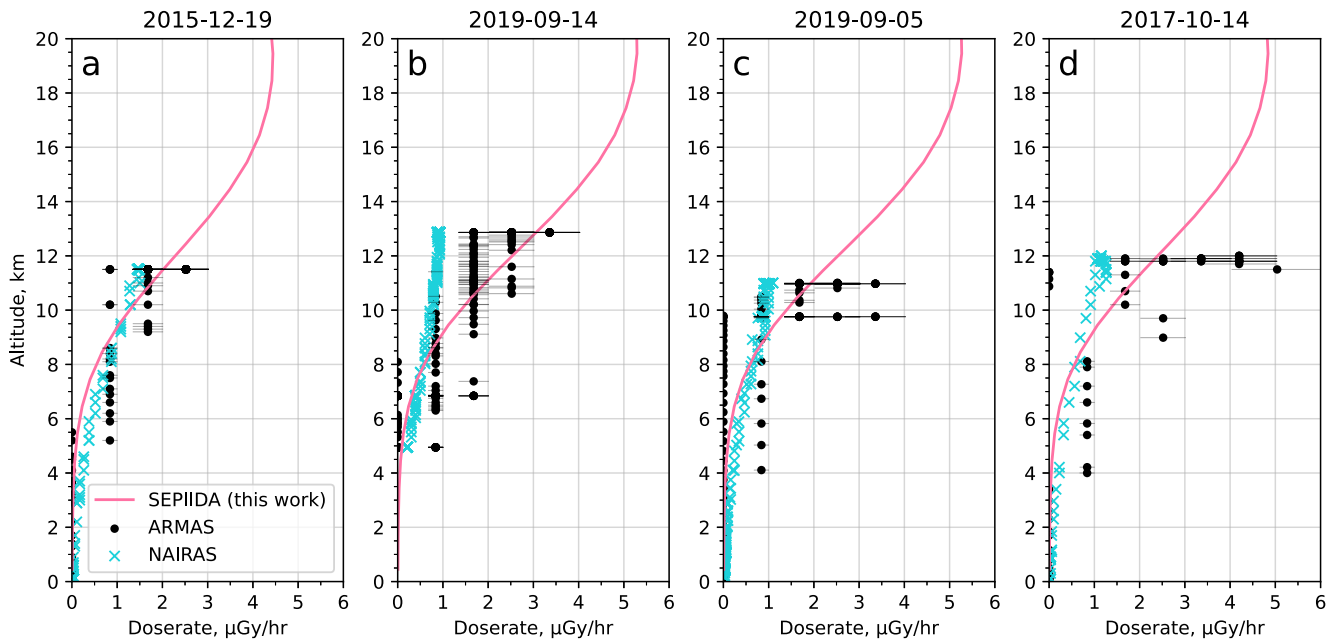
Figure 4. Four example conjunction dates between ARMAS and AMS-02 showing the ARMAS-measured dose rate (black dots), NAIRAS v1-predicted GCR dose rate (blue crosses), and our predicted GCR dose rate based on AMS-02 data (pink line).
