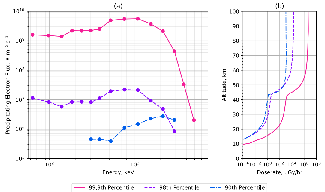
Figure 7. (a) Precipitating electron spectra derived from ELFIN-measured datapoints at the 99.9th (solid magenta line), 98th (dashed purple line), and 90th (dash-dotted blue line) percentile of supra-MeV electron precipitation events recorded by ELFIN. (b) Dose rate in a silicon detector due to each of the spectra in (a) as a function of altitude.
