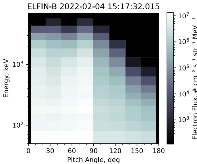
Figure 6. Example of one timestep (1.4 s) of ELFIN data. Data was recorded in the northern hemisphere with a loss cone angle of approximately 68^\circ .
