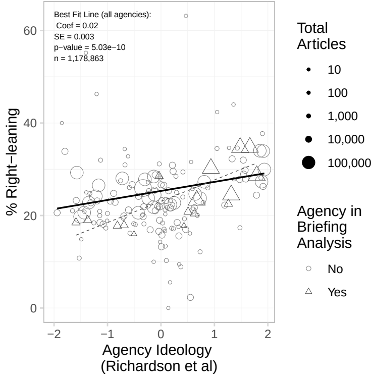
Figure 5: Supply of partisan news about government agencies. Includes articles that mention agencies with ideology scores during 85 randomly sampled weeks from 2015-2025. Standard errors calculated using heteroskedasticity-robust standard errors and clustering by agency, news source, and article URL.
