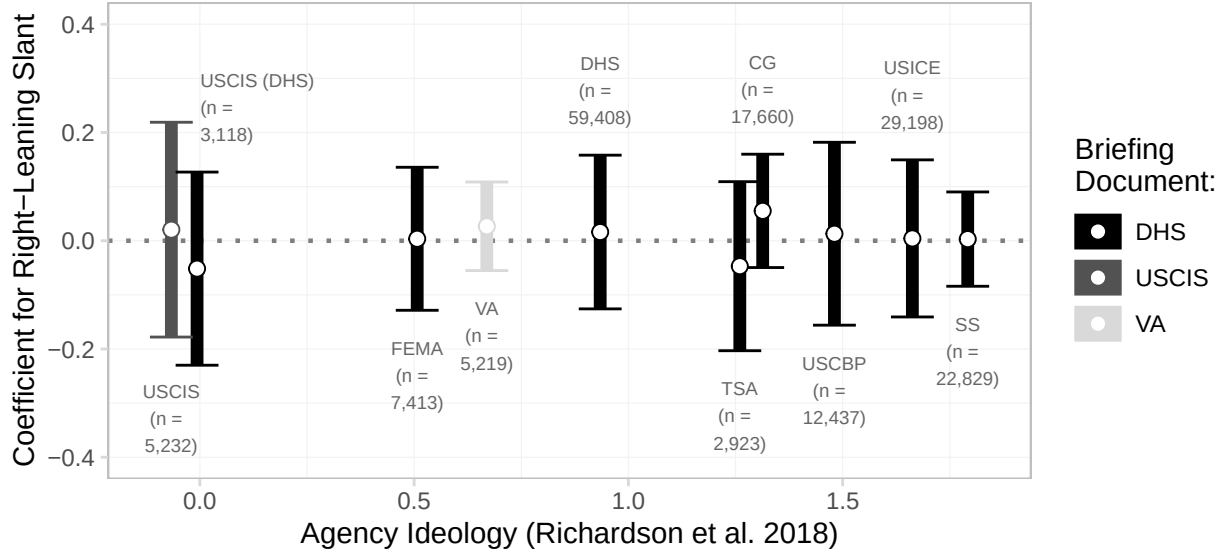
Figure 4: Estimated effect of right-leaning slant on the probability that an article is included in the news briefing. 95% confidence intervals. Models use OLS with robust standard errors clustered by news source and article URL. Outcome variable is binary indicator (1 if article included in news briefing, 0 otherwise). Independent variable is media slant; left-leaning sources are the reference category.
