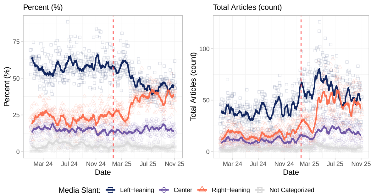
Figure 6: Over-time partisan composition of the DHS news briefings. Dotted line at Trump’s 2025 inauguration. Lines are 2-week rolling averages.
