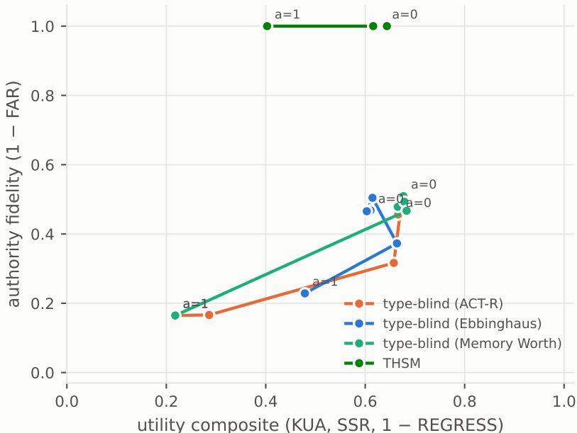
Utility-authority frontier under decay (gpt-4o-mini)
