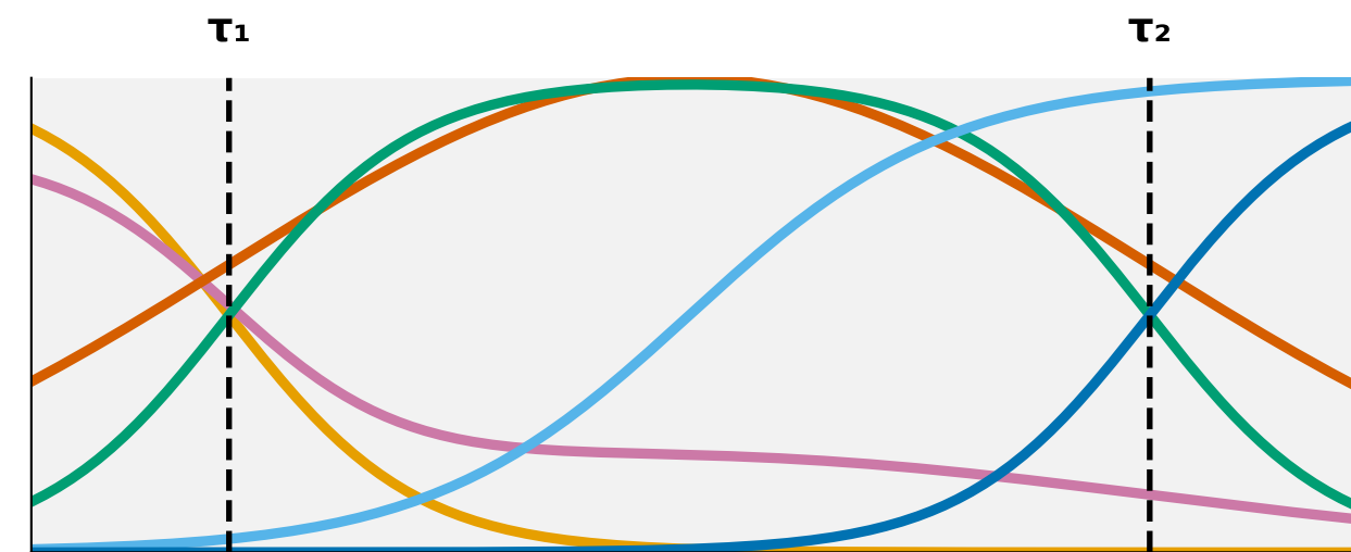
CIFAR-100
