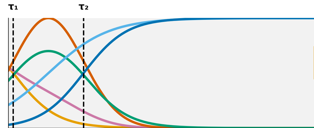
CIFAR-100+SimCLR
