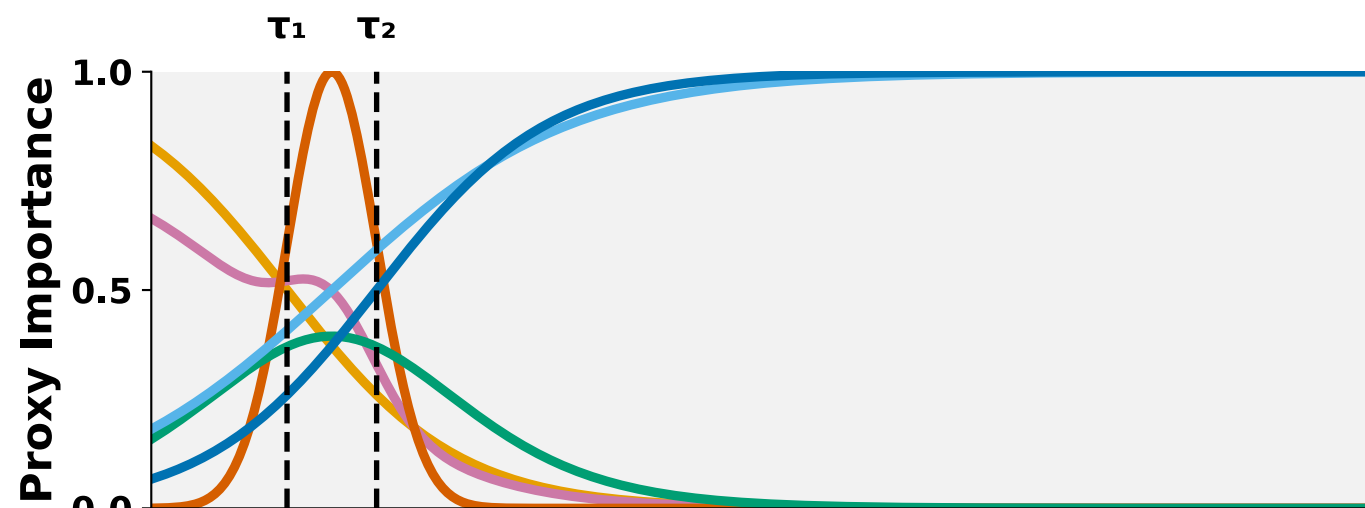
CIFAR-10
