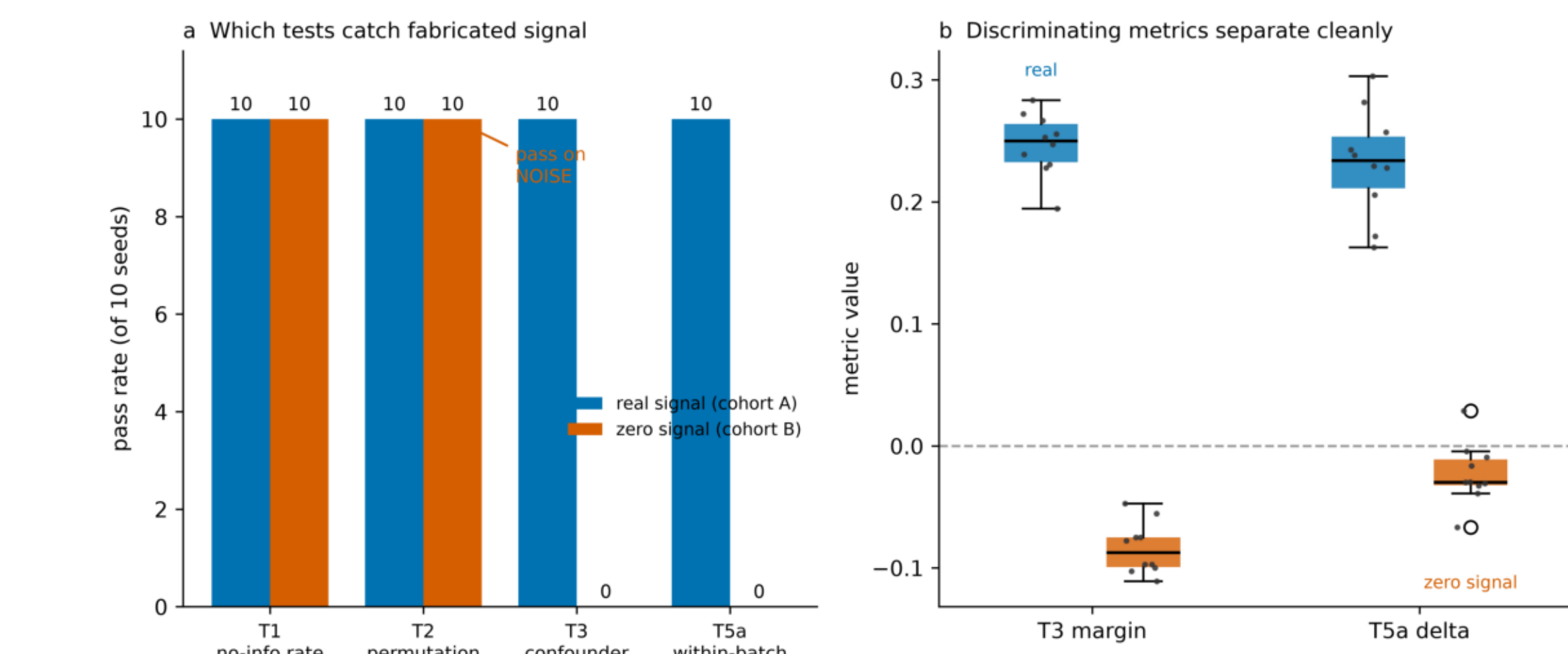
Fig 1 Pass rate by test across ten seeds. T1 and T2 pass in both cohorts; only T3 and T5a separate them.
