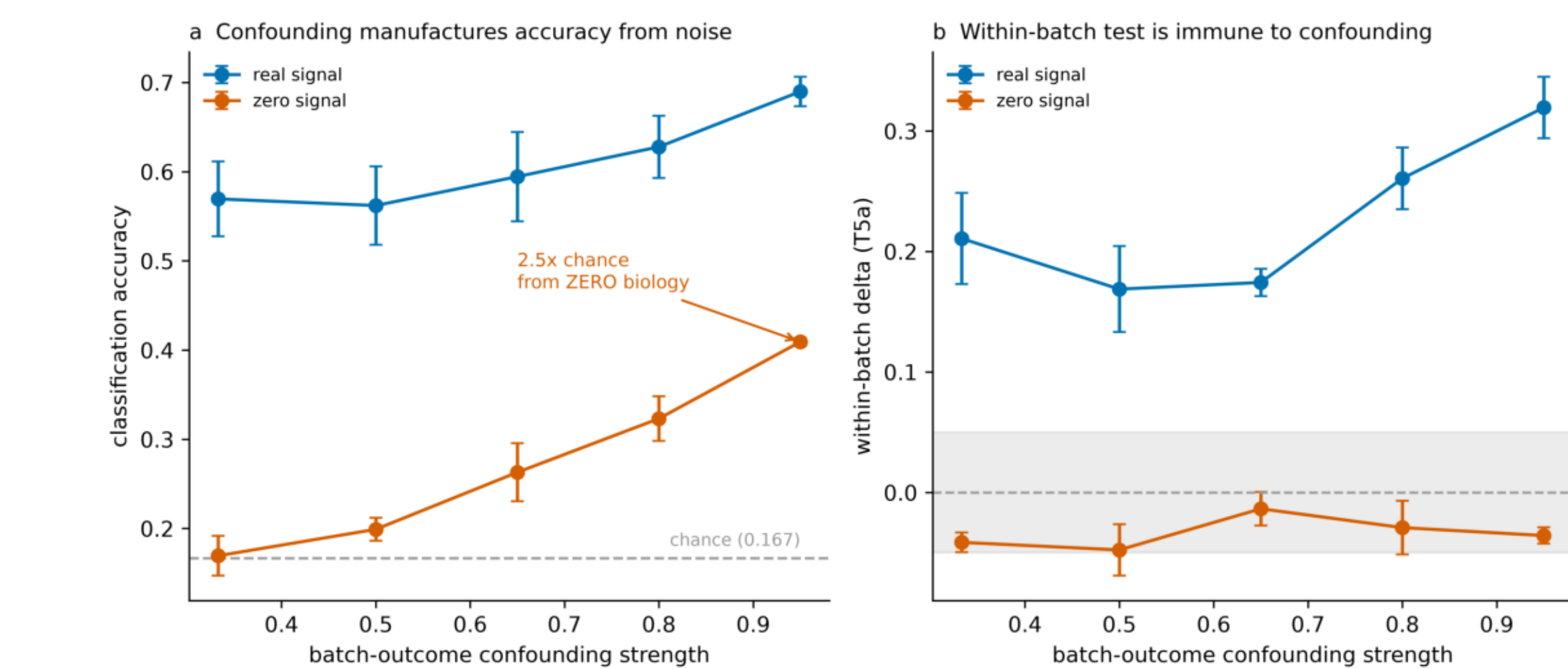
Fig 2 Accuracy against confounding strength. Within-batch delta stays near zero for zero-signal data at every level.
