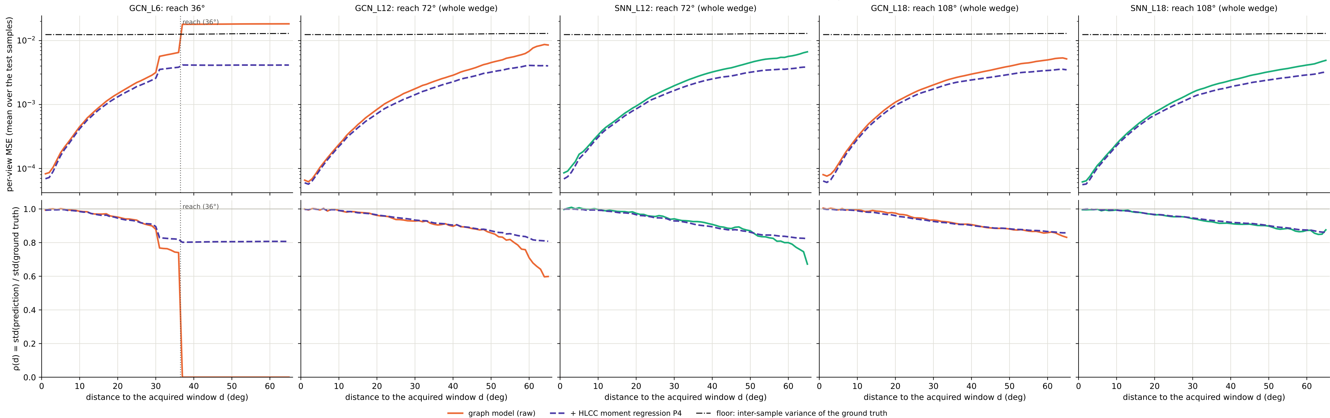
Graph models with and without the HLCC moment regression, vs distance to the acquired window
