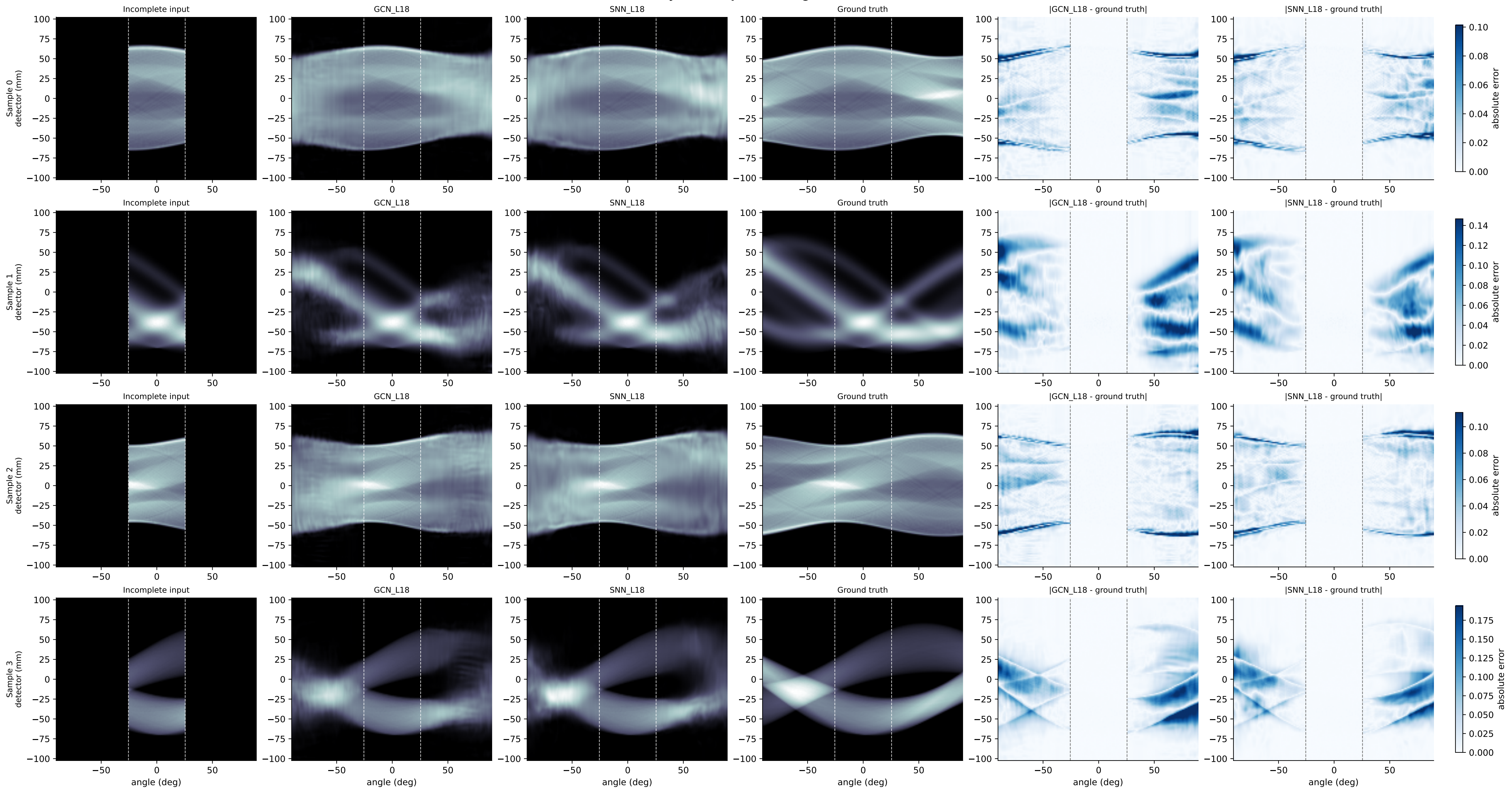
GCN vs SNN at 18 layers: completed sinograms and absolute errors
