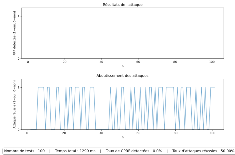
FIGURE 9 – Attack on the hashed version with SHA-256
